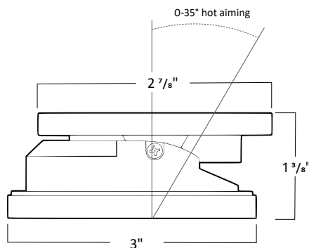
Adjustable Module Holder
