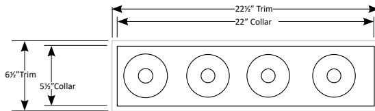
Four module
